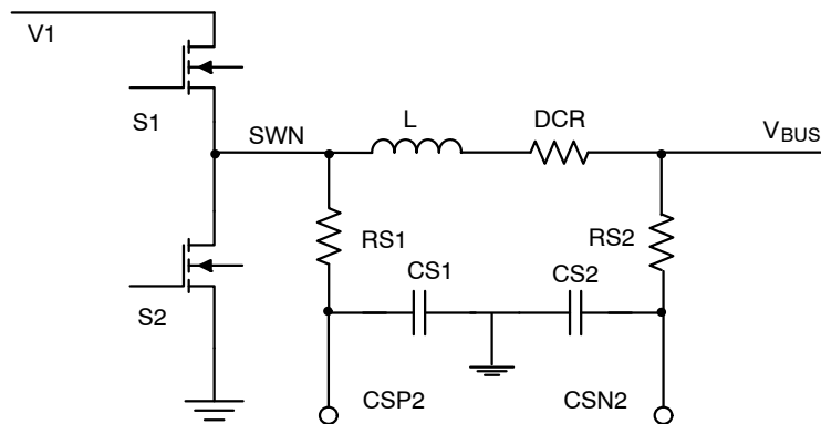
Figure 15. Inductor DCR Sensing Using CSP2/CSN2
