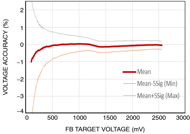
Figure 5. Reference Voltage Accuracy at Temperature -40°C
