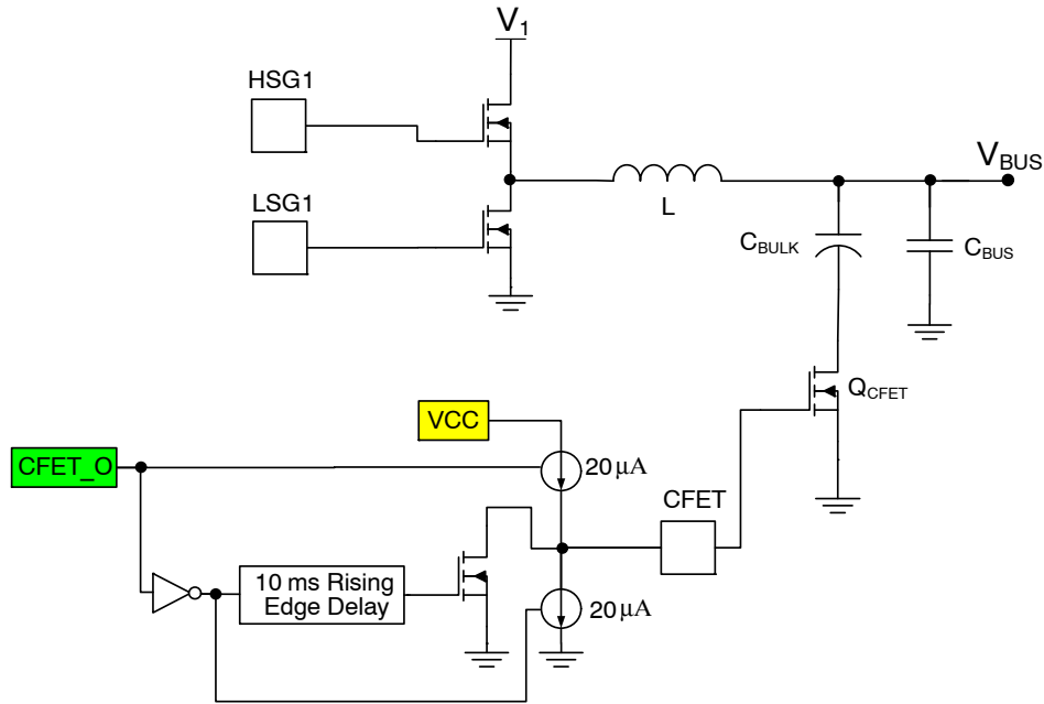
Figure 19. CFET Drive
