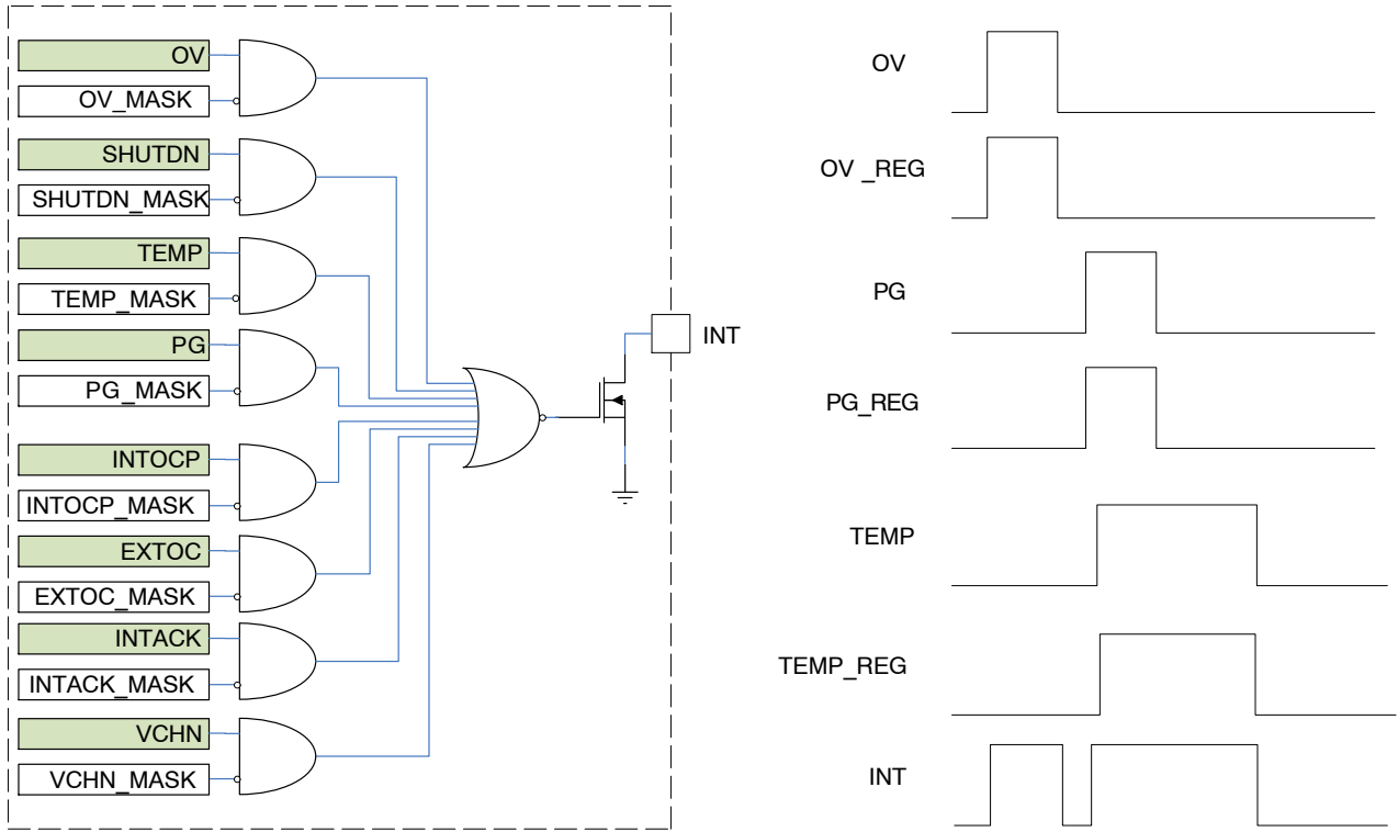
Figure 22. Interrupt Logic
