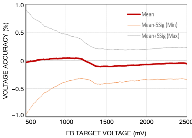
Figure 9. Reference Voltage Accuracy at Temperature 85°C
