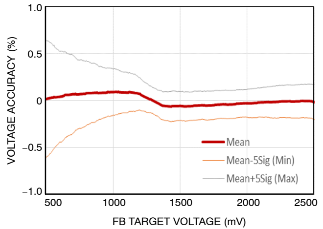
Figure 8. Reference Voltage Accuracy at Temperature 55°C
