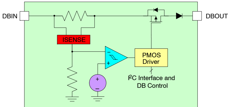
Figure 28. Dead Battery Control Circuitry
