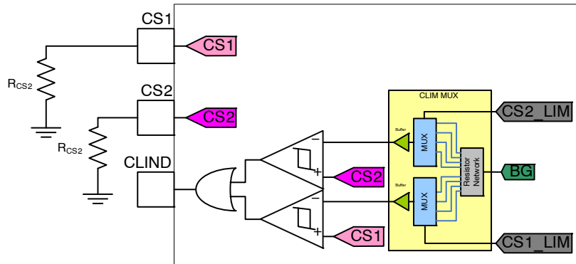
Figure 16. Block Diagram for CLIM Comparator
