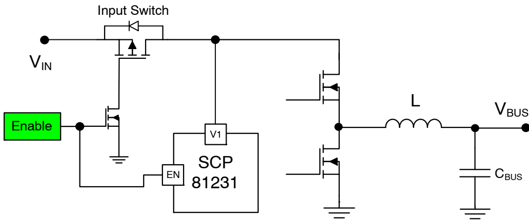
Figure 13. Input Switch Circuit to Disconnect V1 when EN is Low
