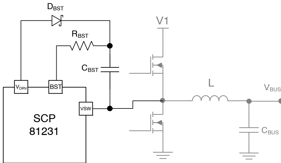
Figure 30. Bootstrap Circuit with Recommended Resistor R_{BST}
