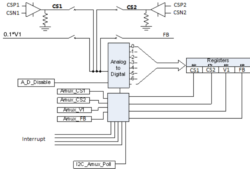
Figure 21. Analog to Digital Converter
