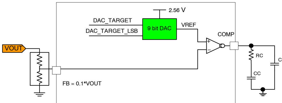
Figure 11. Slew Rate Limiting Block Diagram and Waveforms
