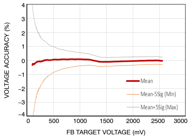
Figure 10. Reference Voltage Accuracy at Temperature 105°C
