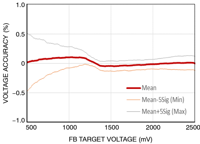
Figure 7. Reference Voltage Accuracy at Temperature 25°C
