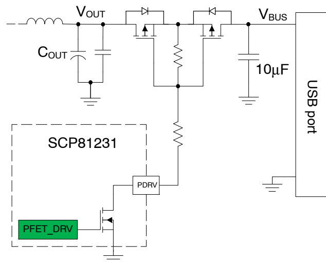
Figure 20. PFET Drive
