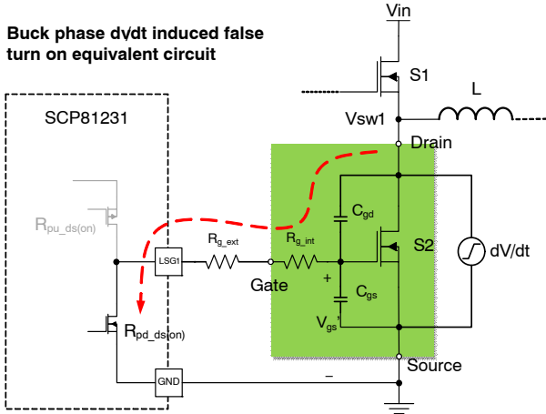
Figure 29. dv/dt Induced False Turn-on Equivalent Circuit of a Buck Converter
