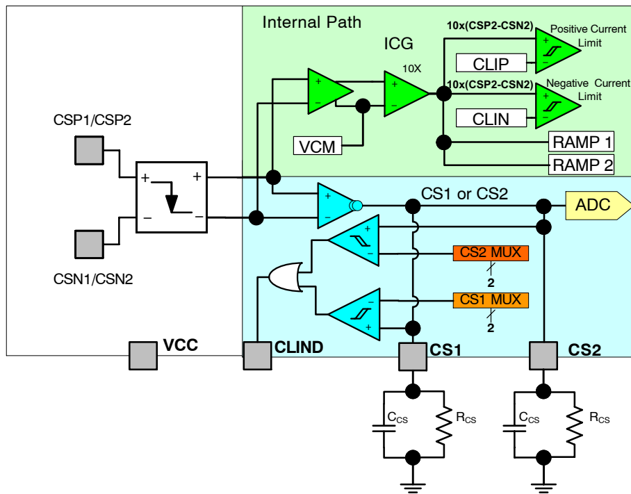
Figure 14. Block Diagram for Current Sense Channel
