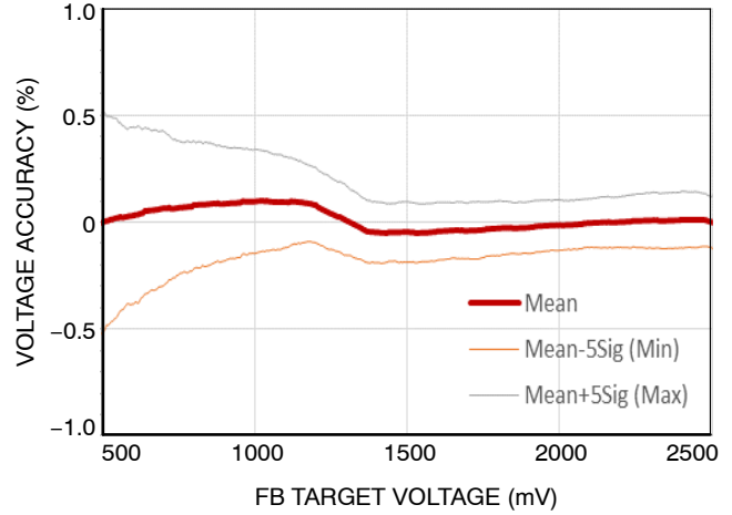
Figure 6. Reference Voltage Accuracy at Temperature 0°C
