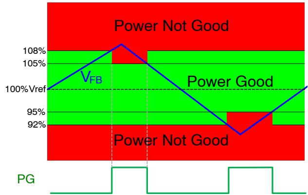
Figure 18. PG Diagram
