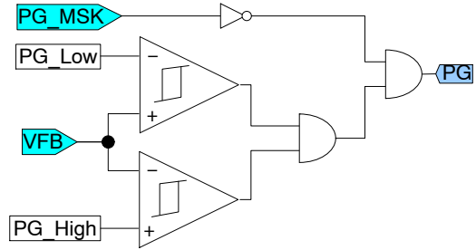
Figure 17. PG Block Diagram
