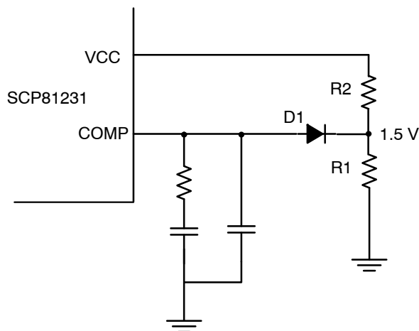
Figure 12. External Comp Clamping Circuit
