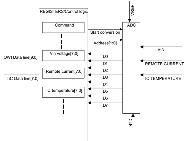
Figure 8. ADC diagram
