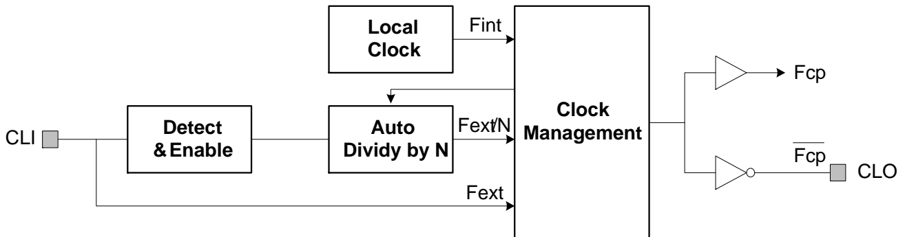
Figure 5. CLI/CLO Schematic
