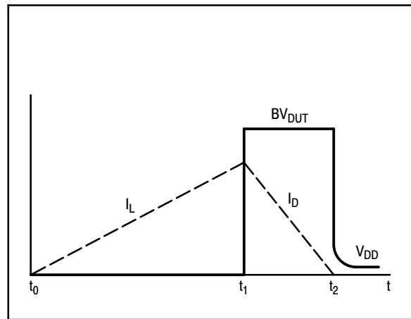
Figure 7. Current–Voltage Waveforms
