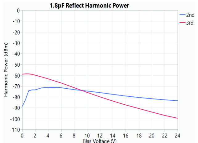
Figure 3. Harmonic Power*
