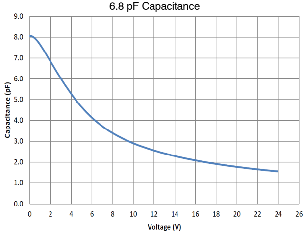
Figure 2. Capacitance
