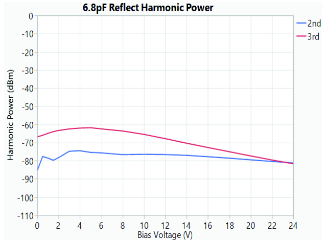
Figure 3. Harmonic Power*
