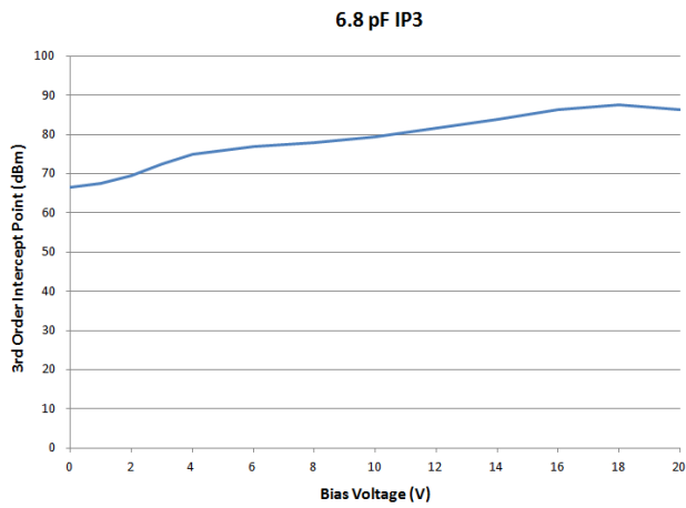
Figure 4. IP3*
