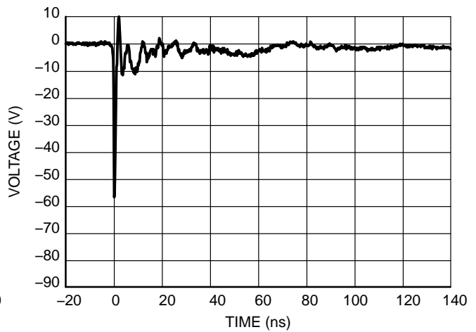
Figure 7. IEC61000-2-4 -8 kV Contact Clamping Voltage
