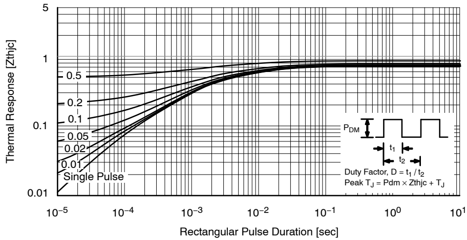
Figure 21. Transient Thermal Impedance of Diode
