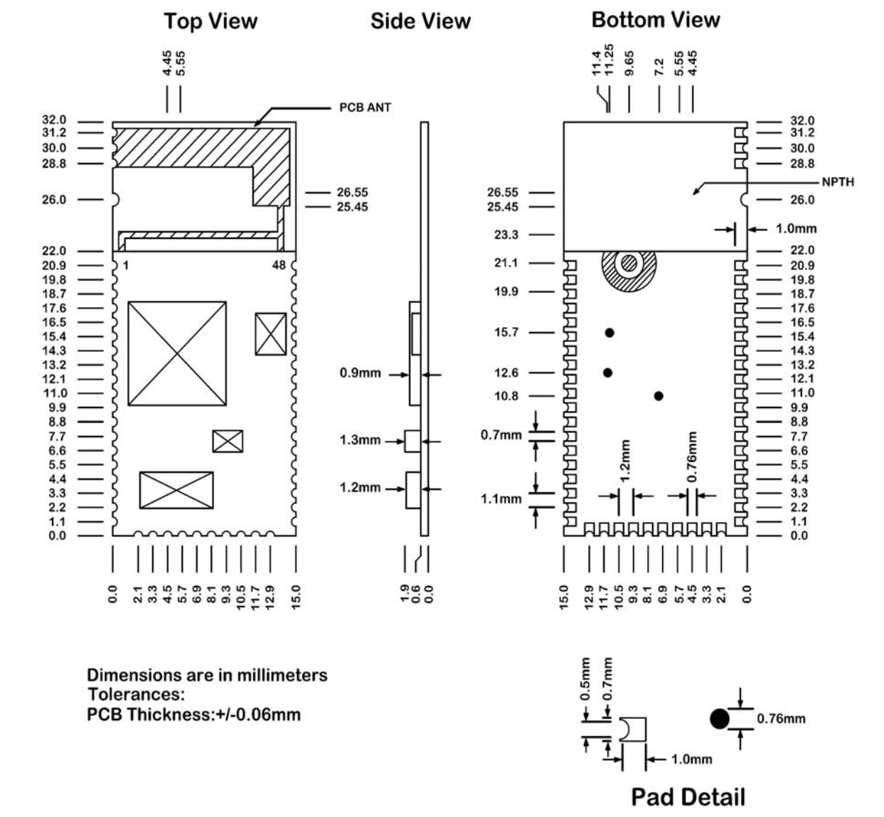
FIGURE 3: BM63 PCB DIMENSION
