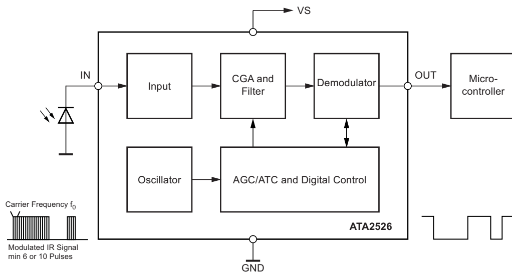
Figure 1-1. Block Diagram
