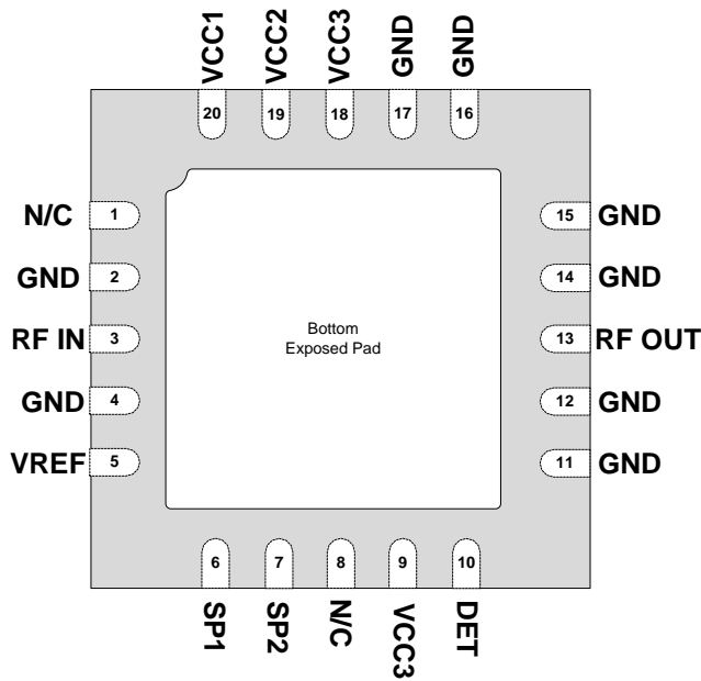
(Top View) LQ Package RoHS/Pb-free 100% matte tin-lead finish
