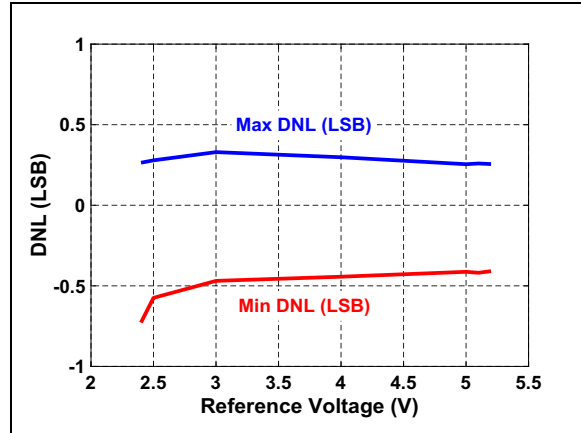
FIGURE 3-10: DNL vs. Reference Voltage.
