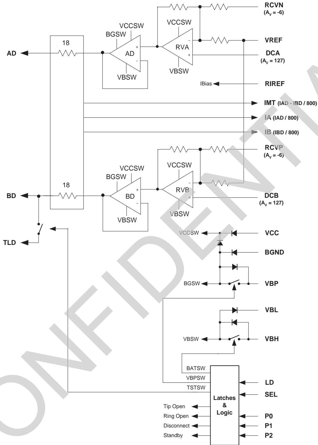
Figure 1. Le79271 Device Internal Block Diagram
