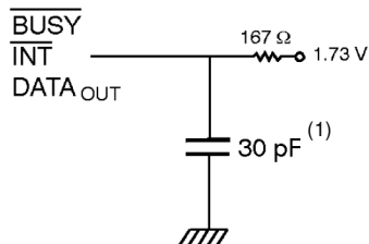
Figure 2. Output Load
