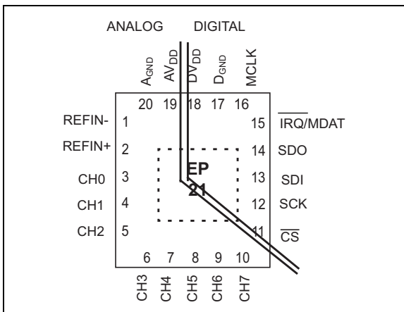
FIGURE 7-7: Separation of Analog and Digital Circuits on the Layout.
