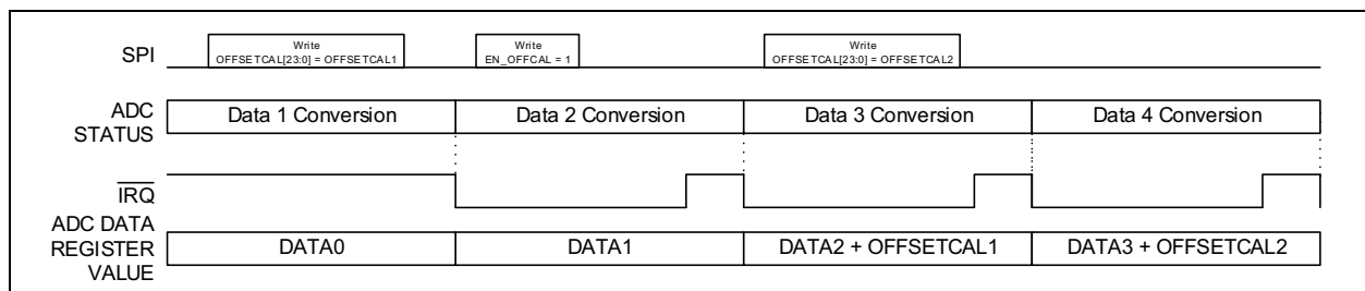
FIGURE 5-11: ADC Output and \overline{IRQ} Behavior with Digital Offset Calibration Enabled.
