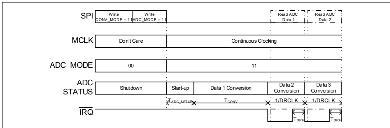
FIGURE 5-14: MUX Continuous Conversion Mode Timing Diagram.
