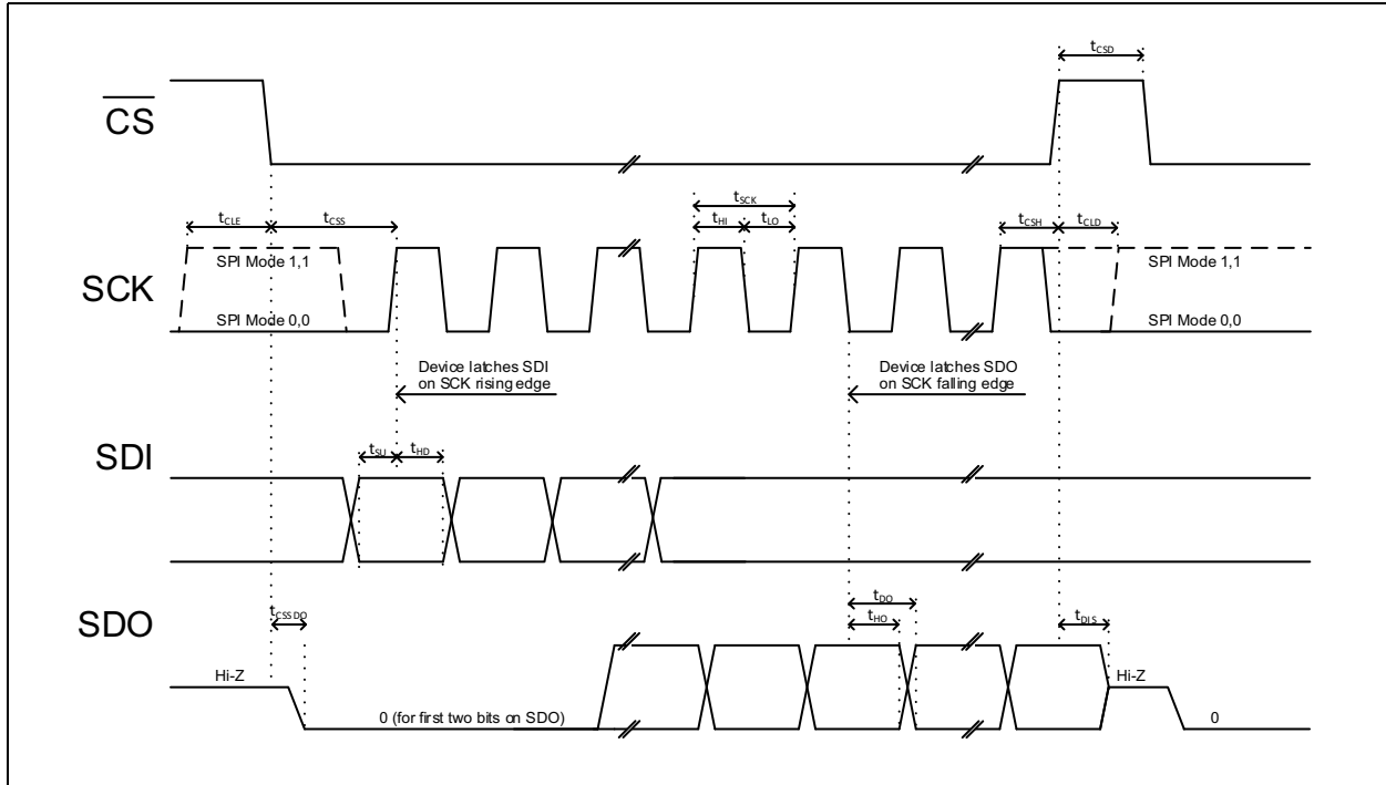
FIGURE 1-1: Serial Output Timing Diagram.
