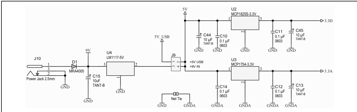
FIGURE 7-6: Power Supply with Separate Lines for Analog and Digital Sections (the "Net Tie" Object Represents the Star Ground Connection).
