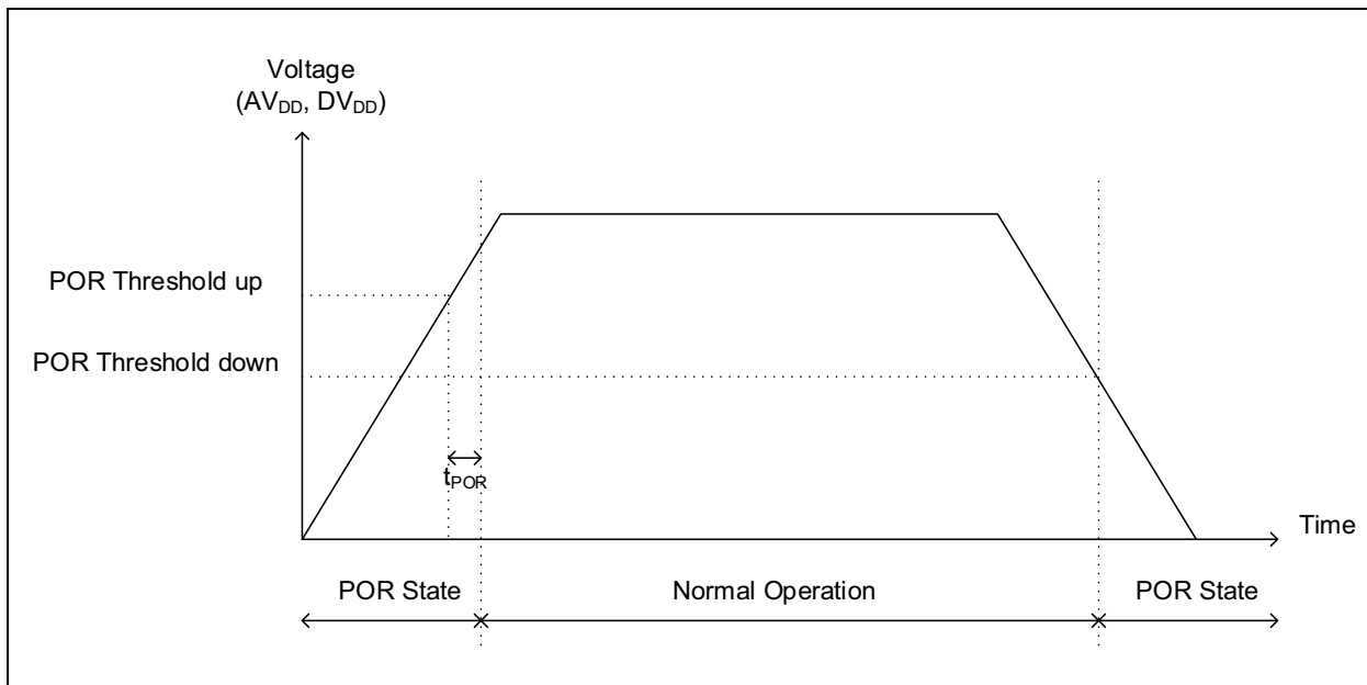
FIGURE 5-9: Power-on Reset Timing Diagram.
