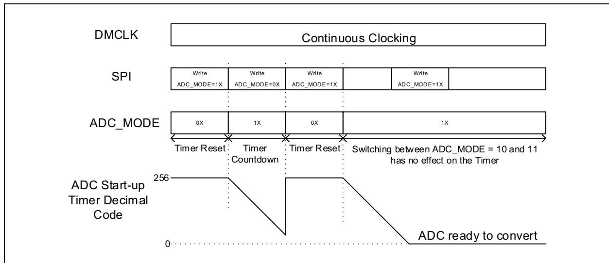
FIGURE 5-10: ADC Start-Up Timer Timing Diagram.
