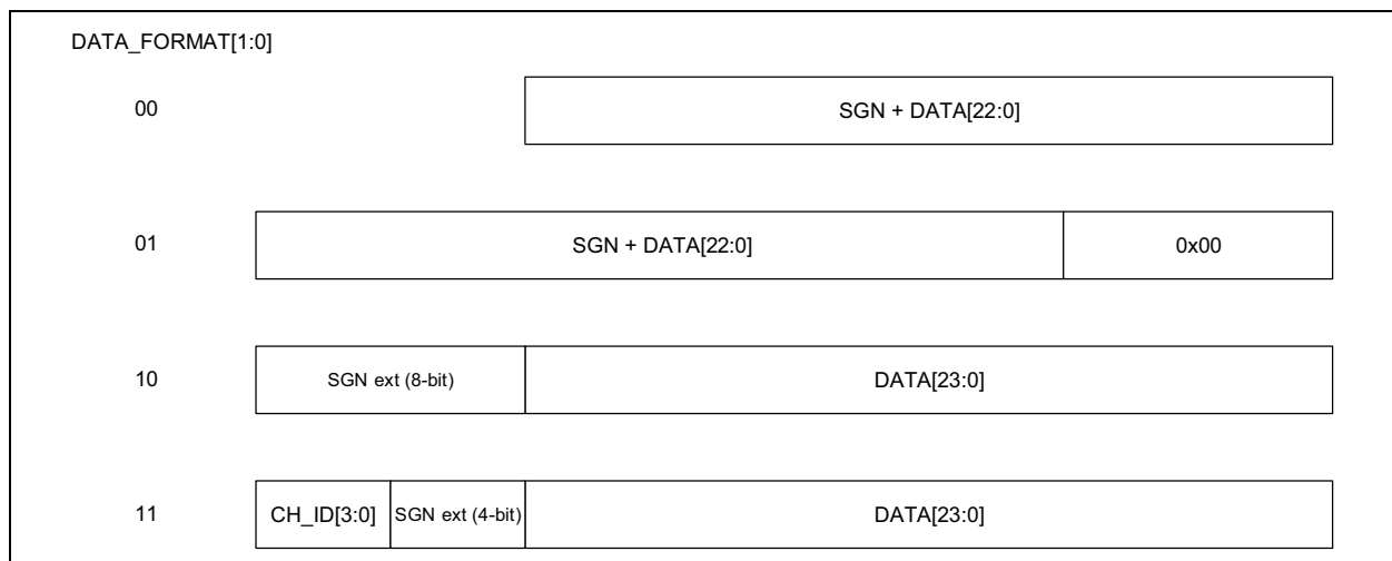
FIGURE 5-8: ADC Output Format Selection.
