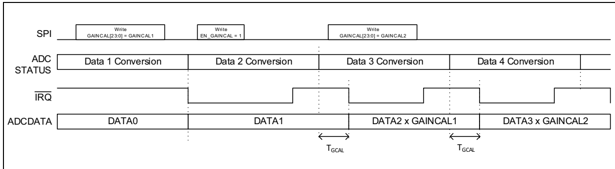
FIGURE 5-12: ADC Output and \overline{IRQ} Behavior with Digital Gain Error Calibration Enabled.
