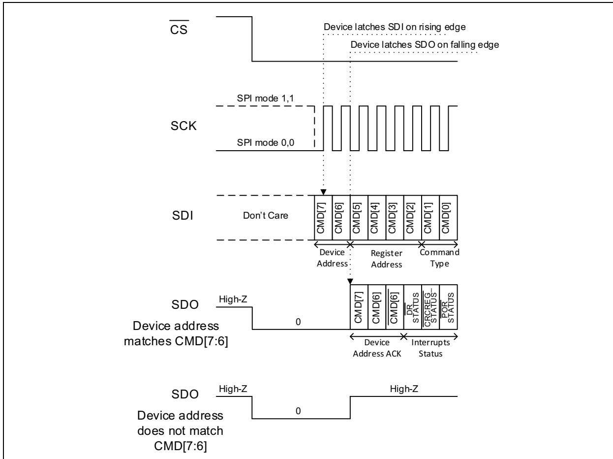
FIGURE 6-2: SPI Communication Start (COMMAND on SDI and STATUS on SDO) when the Device Address Matches/Does Not Match CMD [7:6].
