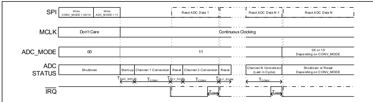
FIGURE 5-15: SCAN One-Shot Conversion Mode Timing Diagram.
