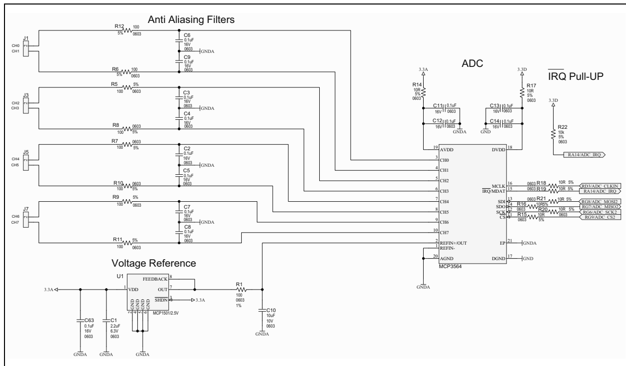
FIGURE 7-1: MCP3564 Application Example.
