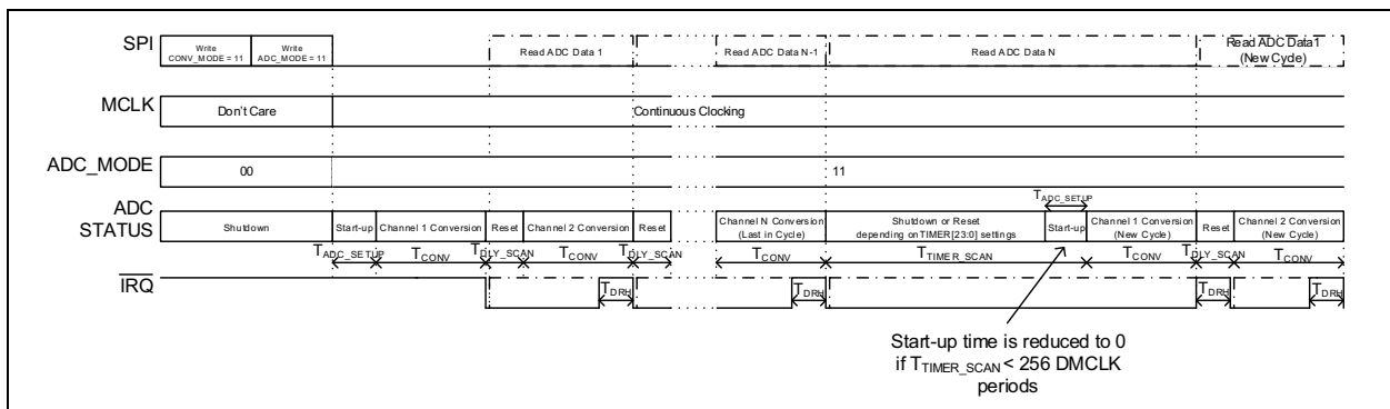
FIGURE 5-16: SCAN Continuous Conversion Mode Timing Diagram.
