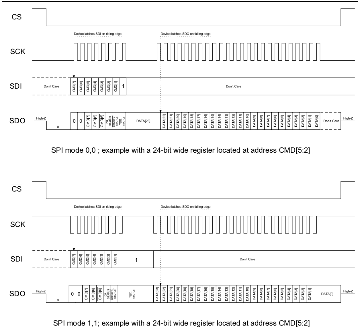
FIGURE 6-7: Single-Read SPI Communication (Static or Incremental Read).
